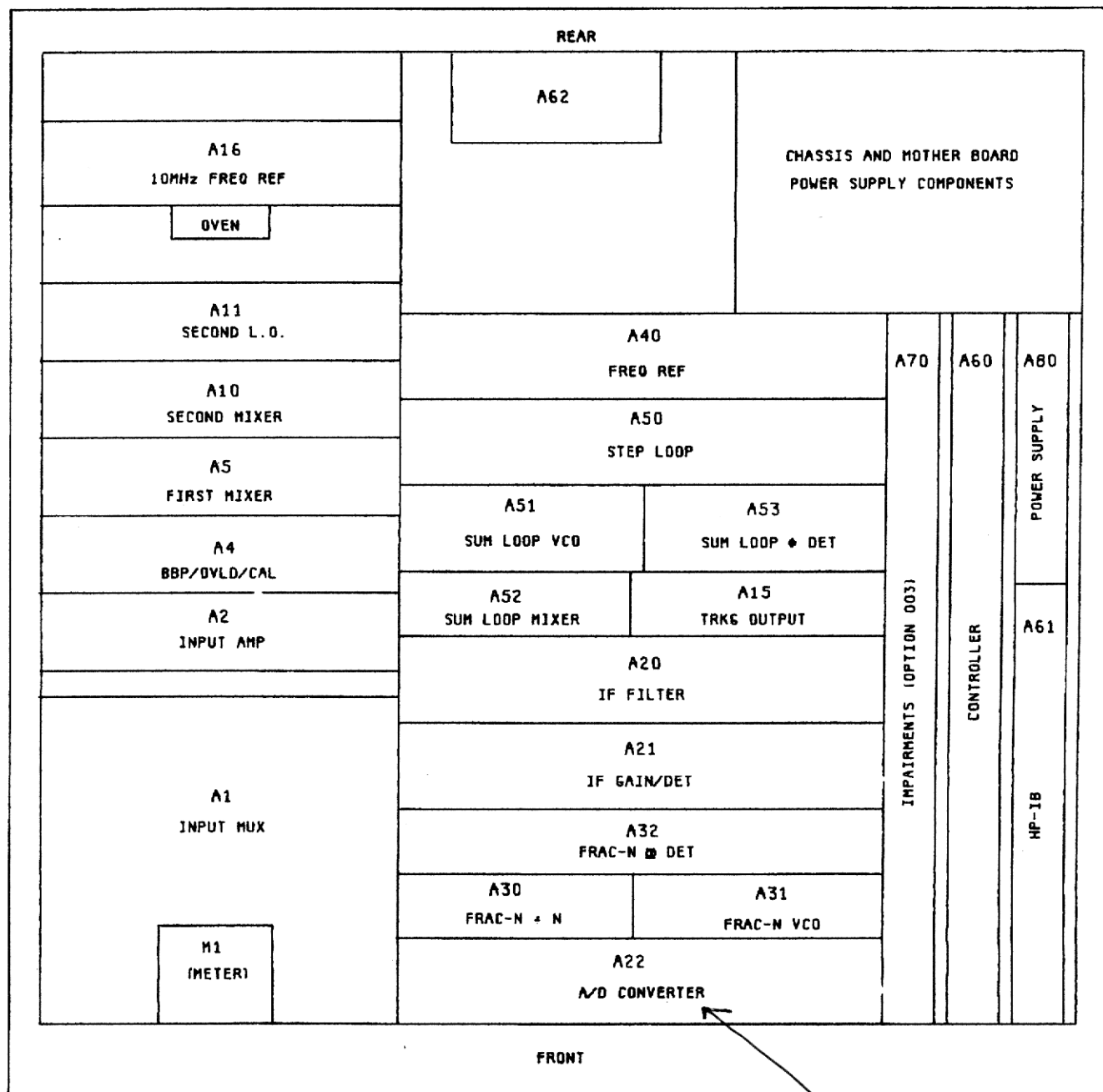
Figure 8-10. Printed Circuit Board Layout.
